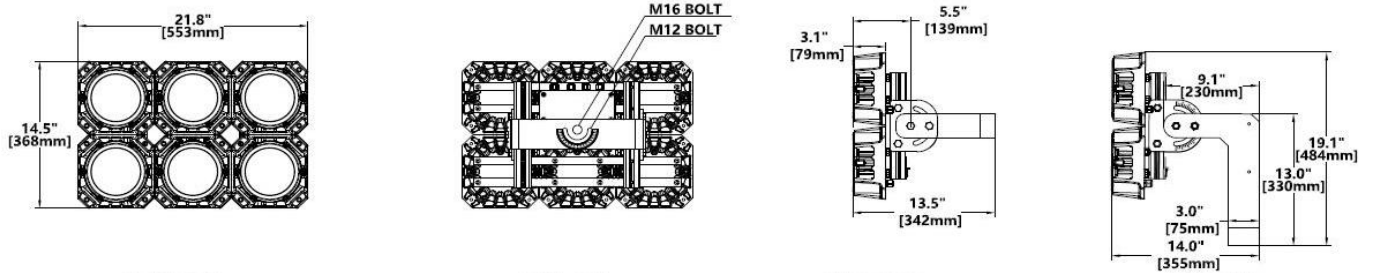
FL12M-840W - 100,800 lumens (Use 2 x FL6M-420W for DLC)
